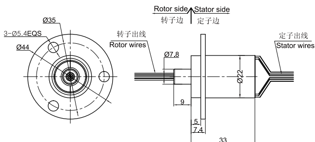
MC330图纸
