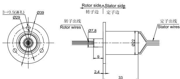
MC330-FL04图纸
