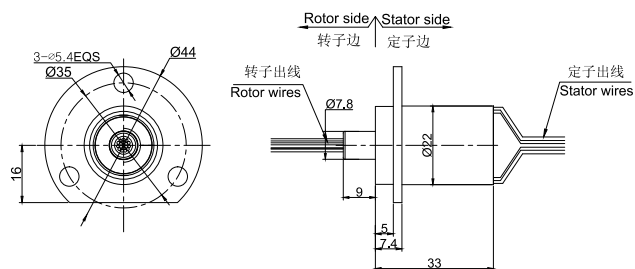
MC330-FL06图纸
