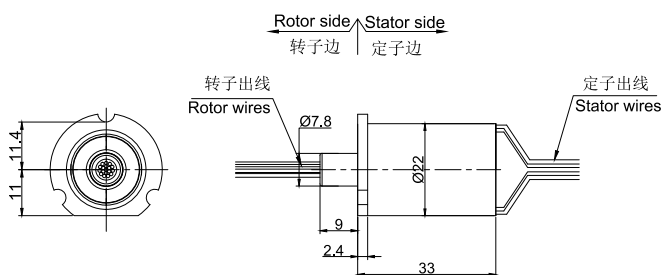
MC330-FL05图纸
