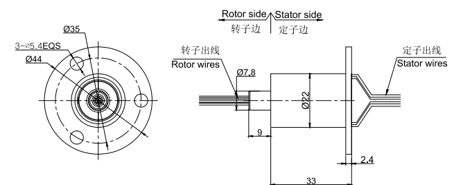
MC330-FL02图纸
