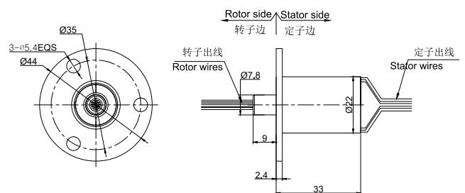
MC330-FL01图纸
