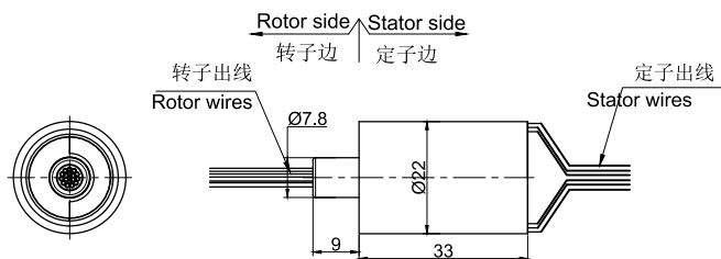
MC330-FL00图纸
