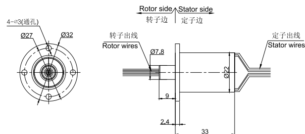
MC330-FL05图纸
